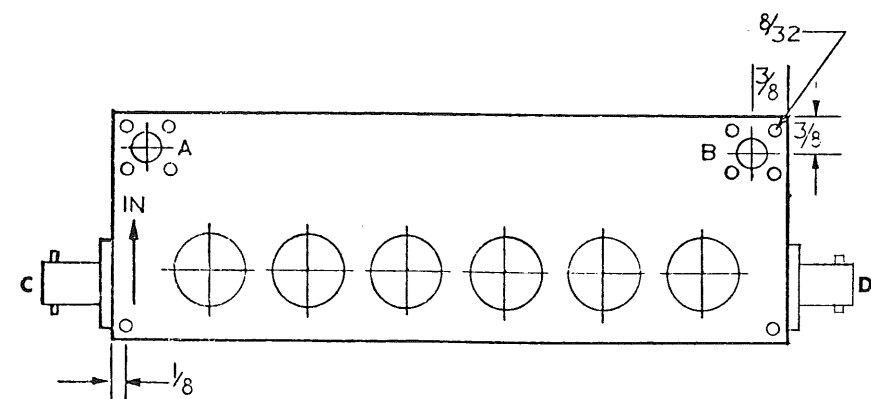
FIG. 2.1 PANEL MOUNTING AND CONNECTOR CONFIGURATION
